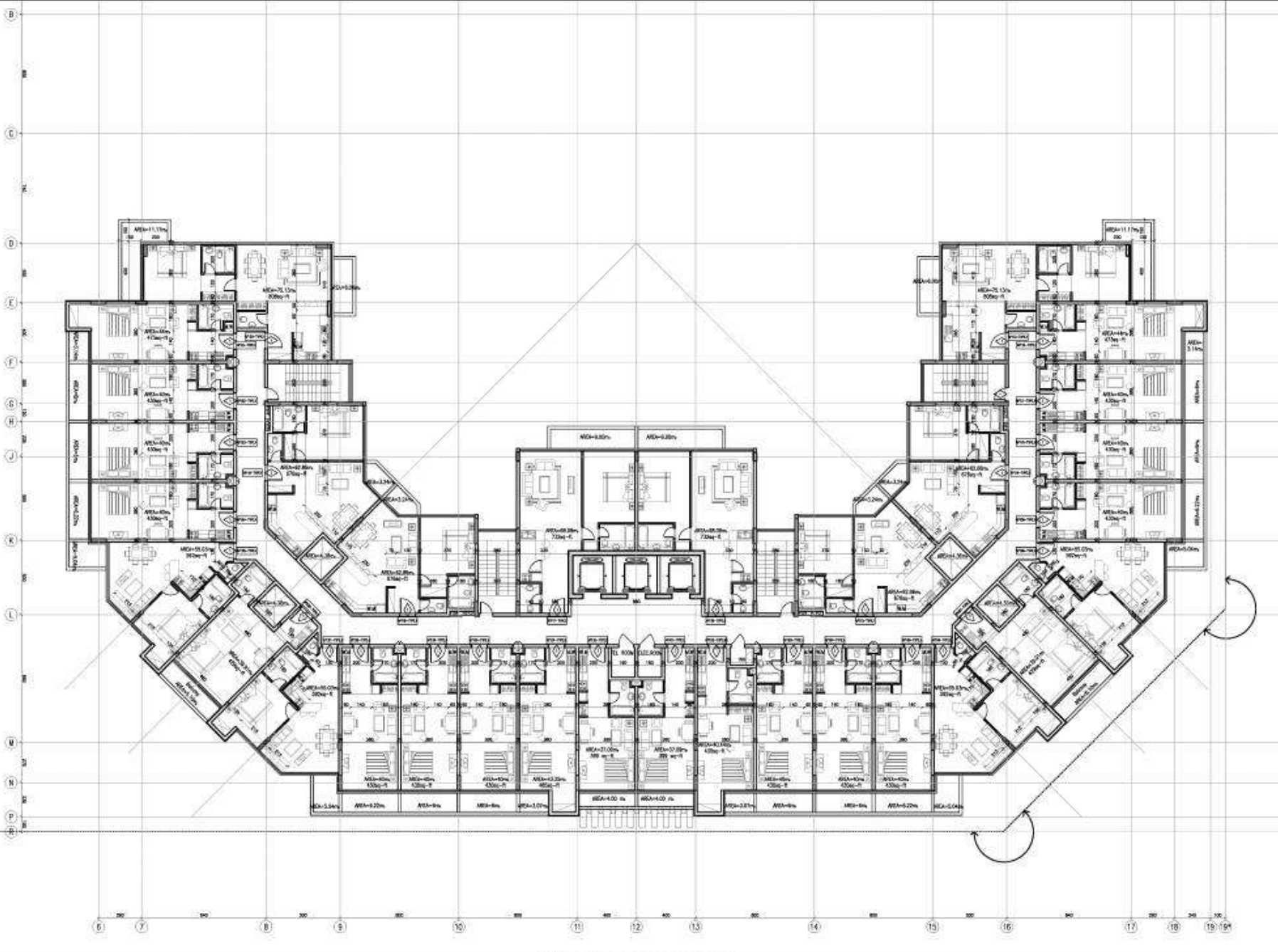
1 st to 8 th FLOOR TYPICAL
